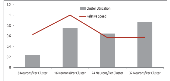
Figure 10: Relative speed of physical neural network versus number of neurons per cluster. Speed is normalized against a default setting of sixteen neurons per cluster. Performance of physical neural network is communication bound when the number of neurons per cluster is small (low cluster utilization). Allocating large number of neurons per cluster increases cluster utilization with reduced concurrency level. For our pipelined neuron cluster, sixteen neurons per cluster achieves the best balance between speed and resource utilization.
