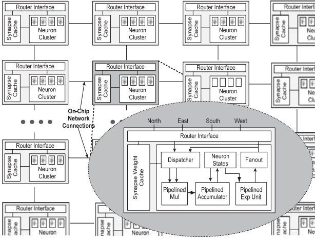
Figure 1: Physical neuron clusters on a single chip: a mesh of physical neuron clusters with on-chip interconnects. Each cluster contains a routing interface for routing neural outputs sent from the neighbors. The functional units of each neuron cluster are pipelined. In addition, each neuron cluster contains a weight cache. Routing is spanning tree based using source neuron cluster identity. Each cluster contains build-in support to reconstruct new spanning trees when permanent faults occur to routing neuron clusters.
