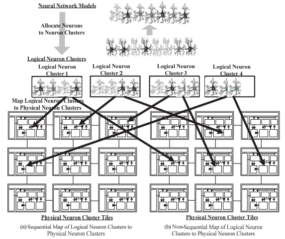
Figure 7: Different approaches of mapping logical neuron clusters to physical neuron clusters: (a) map logical neuron clusters to physical neuron tiles according to a pre-determined pattern; (b) randomly map logical neuron clusters to physical neuron tiles.
